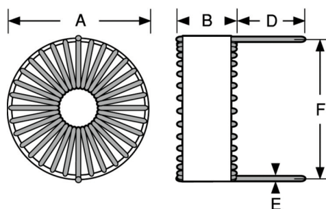
FIGURE 2: HORIZONTAL MOUNT
