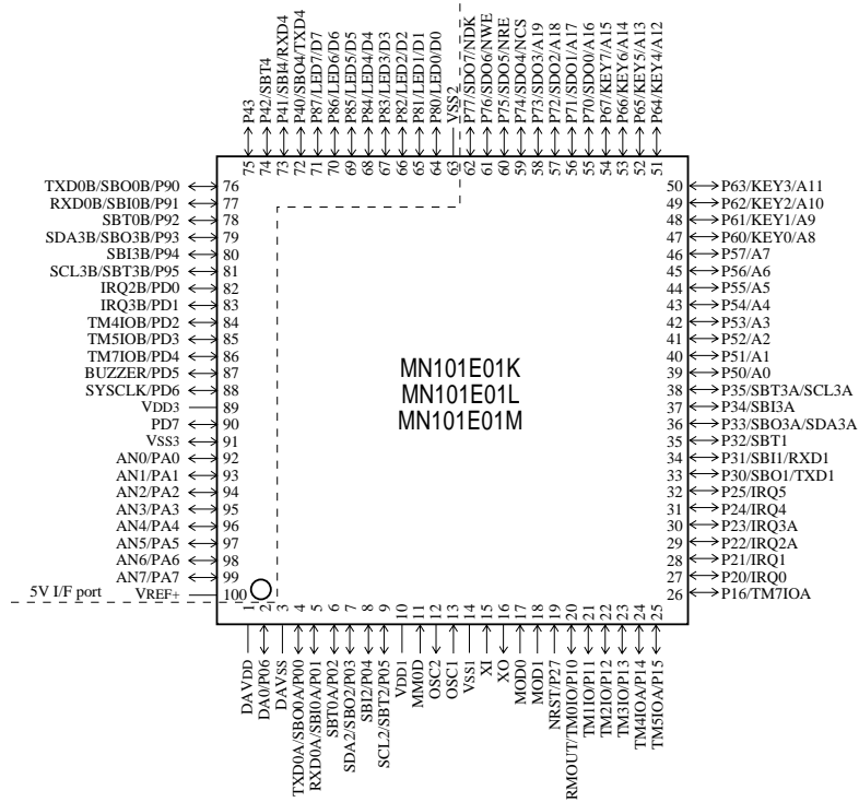
QFP100-P-1818B *Lead-free
