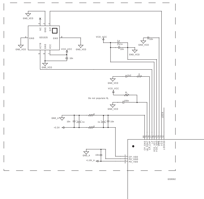
Figure 3-4: Typical Application Circuit using G01525
