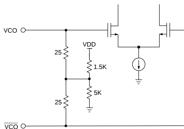
Figure 2-6: VCO Input
