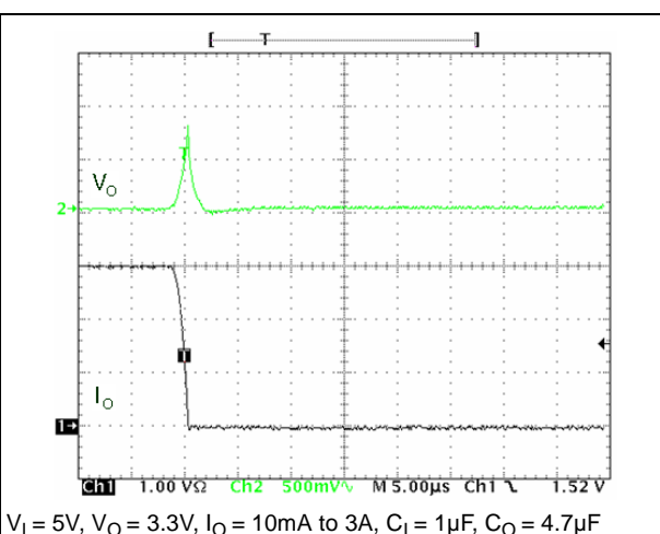
Figure 16. Load transient (fall time)
