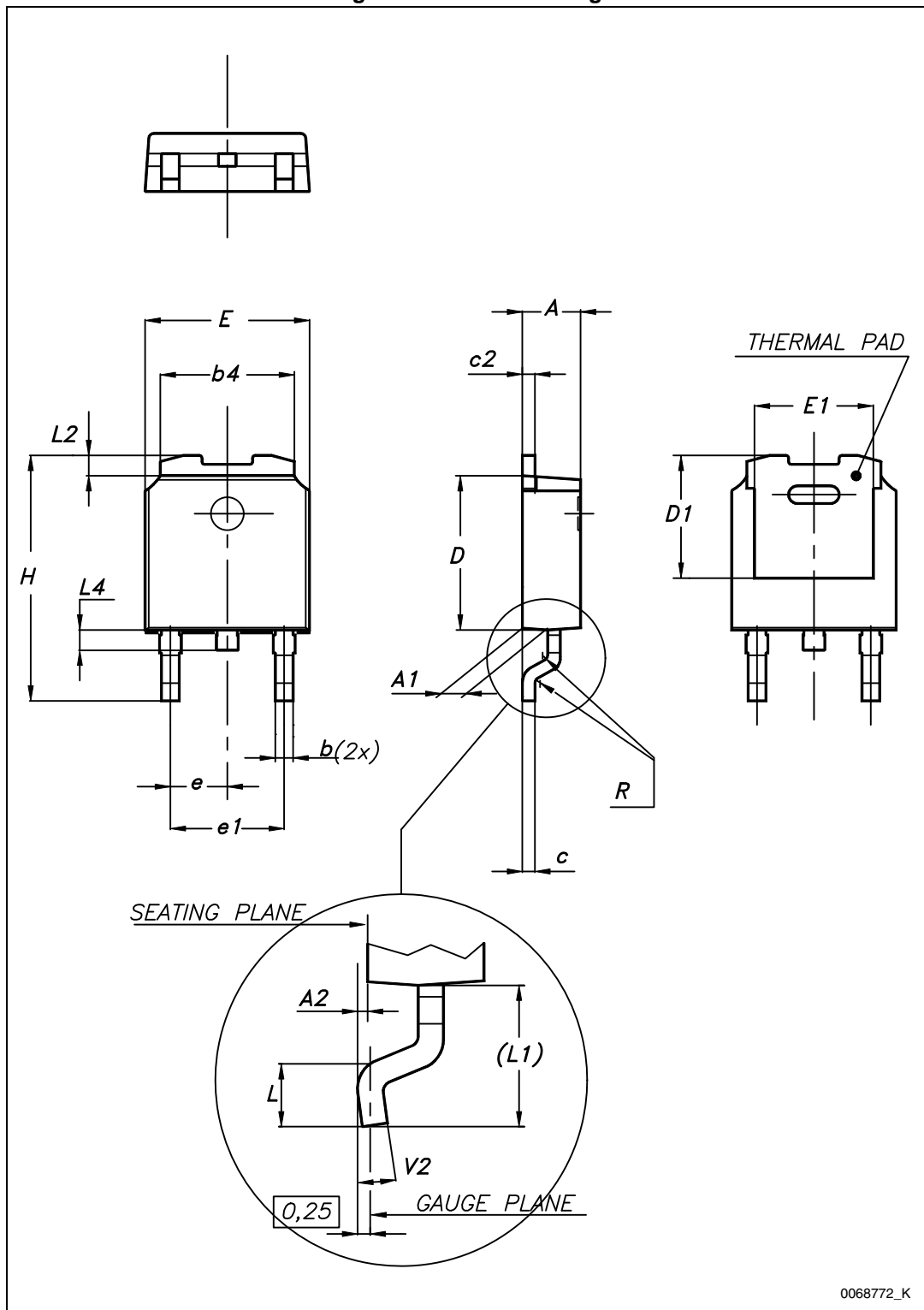
Figure 19. DPAK drawing
