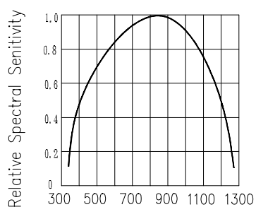
Fig.5 Spectral Sensitivity
