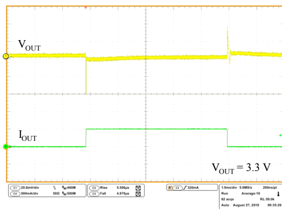
Figure 18. Load transient ( V_{OUT} = 3.3 \text{ V} )
