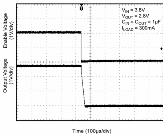
Turn-Off Time
