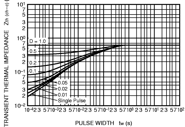
TRANSIENT THERMAL IMPEDANCE CHARACTERISTICS
