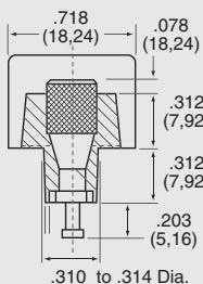
GFTX turret- type solder pin
