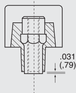
GBSX closed-back design
