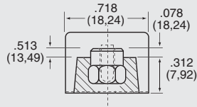
GBFTX turret-type solder pin
