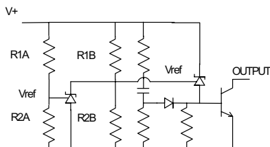
SERIES REGULATOR
