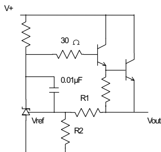
SERIES REGULATOR
