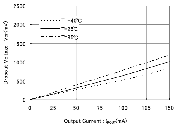
XC6408D/E ( V_{ROUT}=18.0V )
