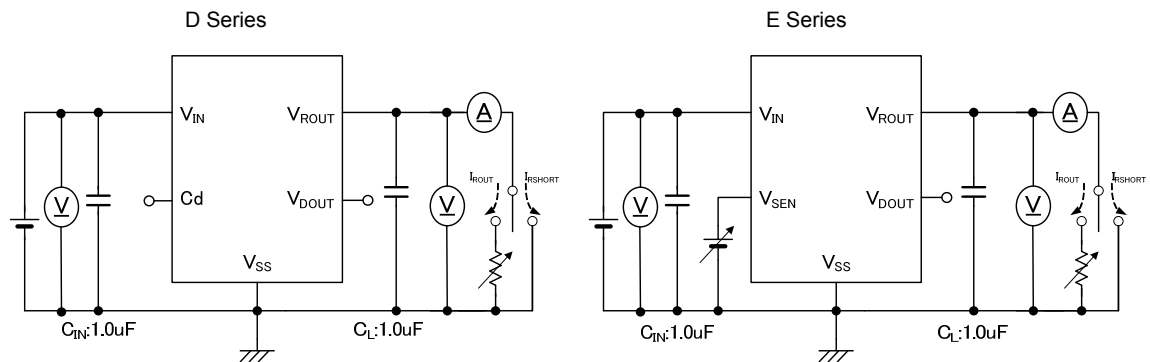
Circuit ②
