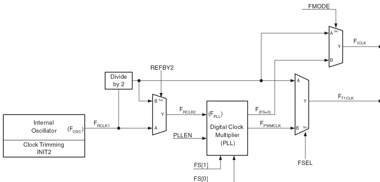
Figure 3. Internal Clock Scheme
