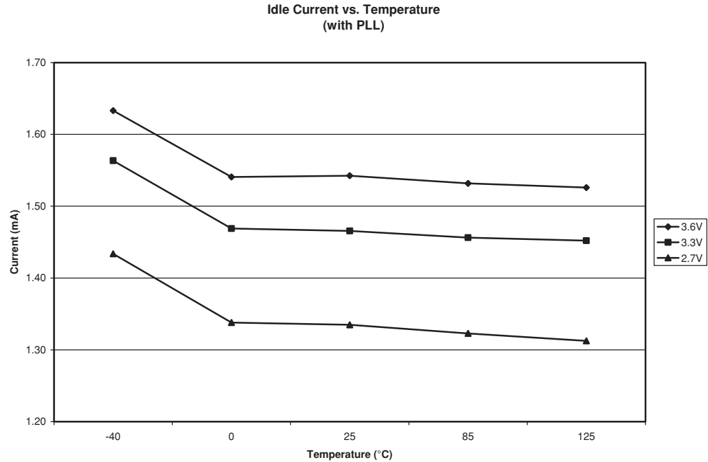
Figure 28. Idle Current vs. Temperature (with PLL)
