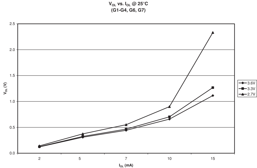
Figure 29. V_{OL} vs. I_{OL} @ 25°C (G1–G4, G6, G7)
