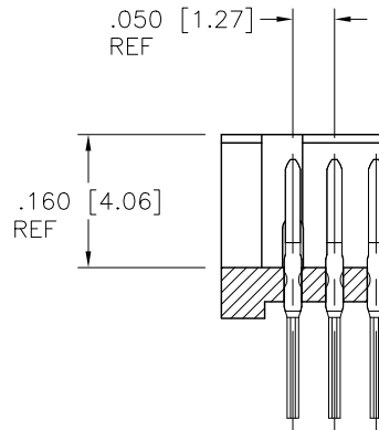
SECTION Y-Y
