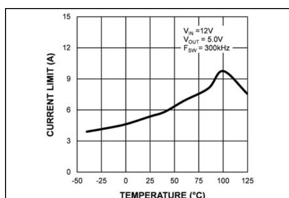
FIGURE 2-24: Output Peak Current Limit vs. Temperature (MIC28511-2).
