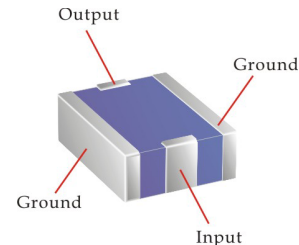
Outline of 3225 size 2.4GHz Bandpass Filter
