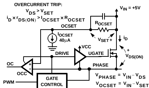
FIGURE 2. OVERCURRENT DETECTION
