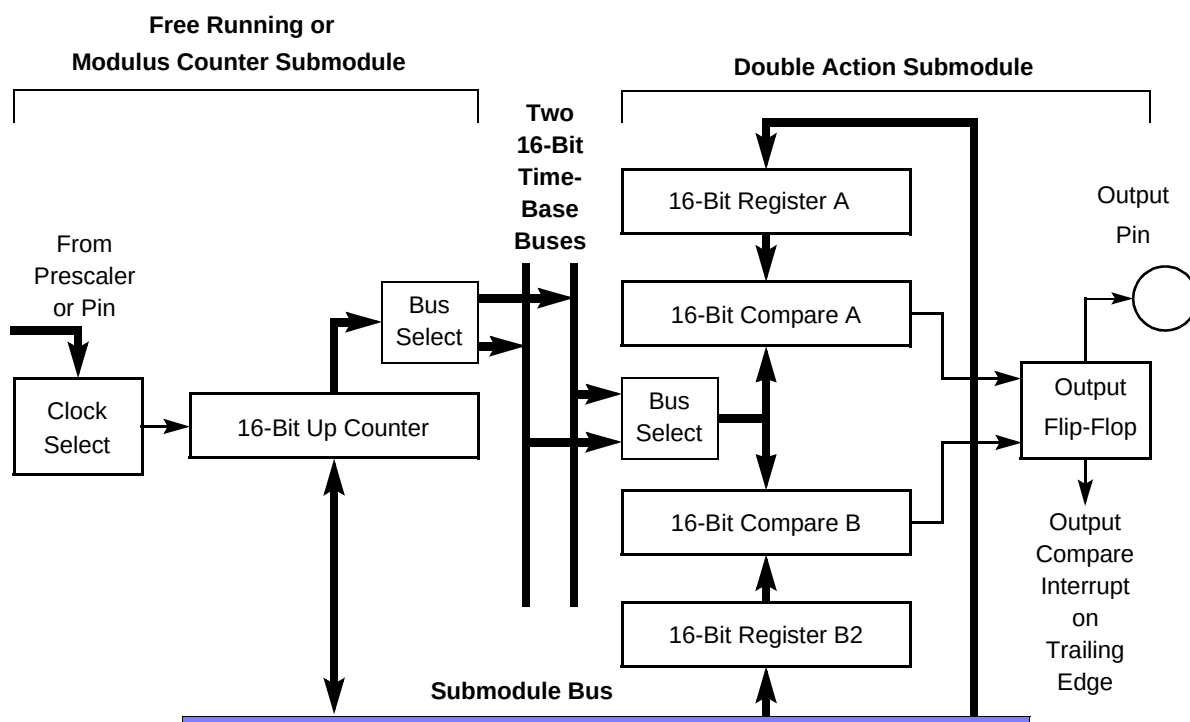
Figure 13-19 CTM9 Example — Double Edge Output Compare
