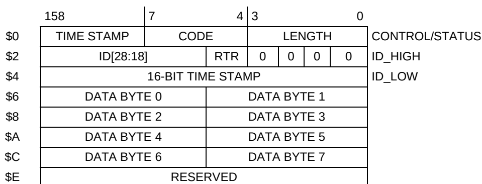
Figure 7-4 Standard ID Message Buffer Structure
