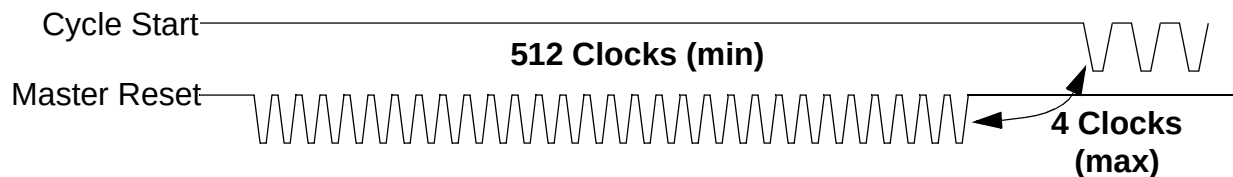
Figure 10-5 Master Reset Configuration Timing
