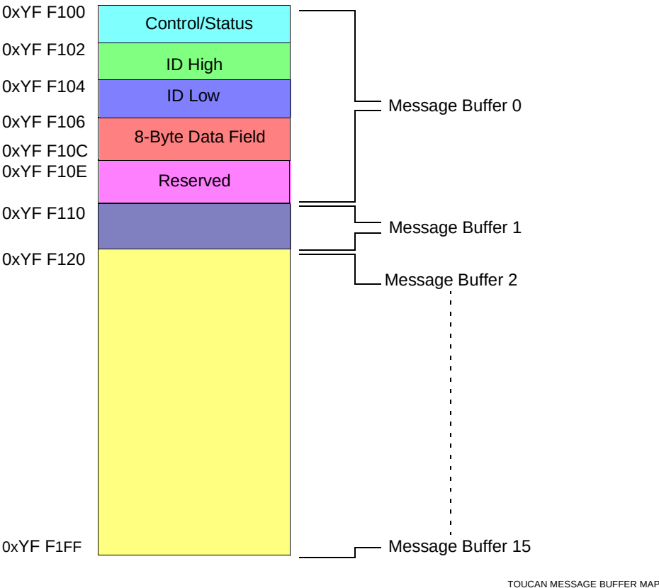
Figure 7-6 TouCAN Message Buffer Memory Map
