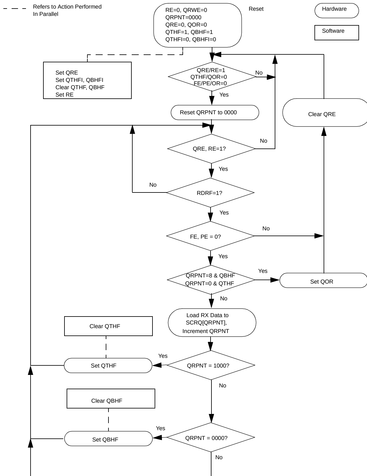
Figure 6-18 Queue Receive Flow
