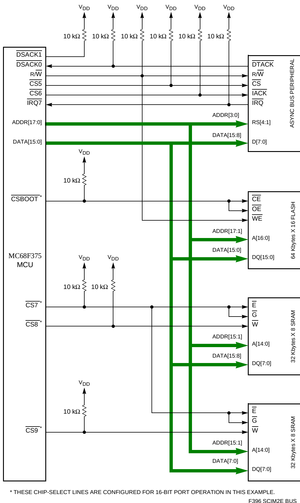
Figure 4-9 MCU Basic System
