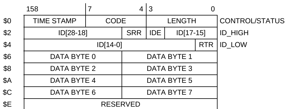
Figure 7-3 Extended ID Message Buffer Structure
