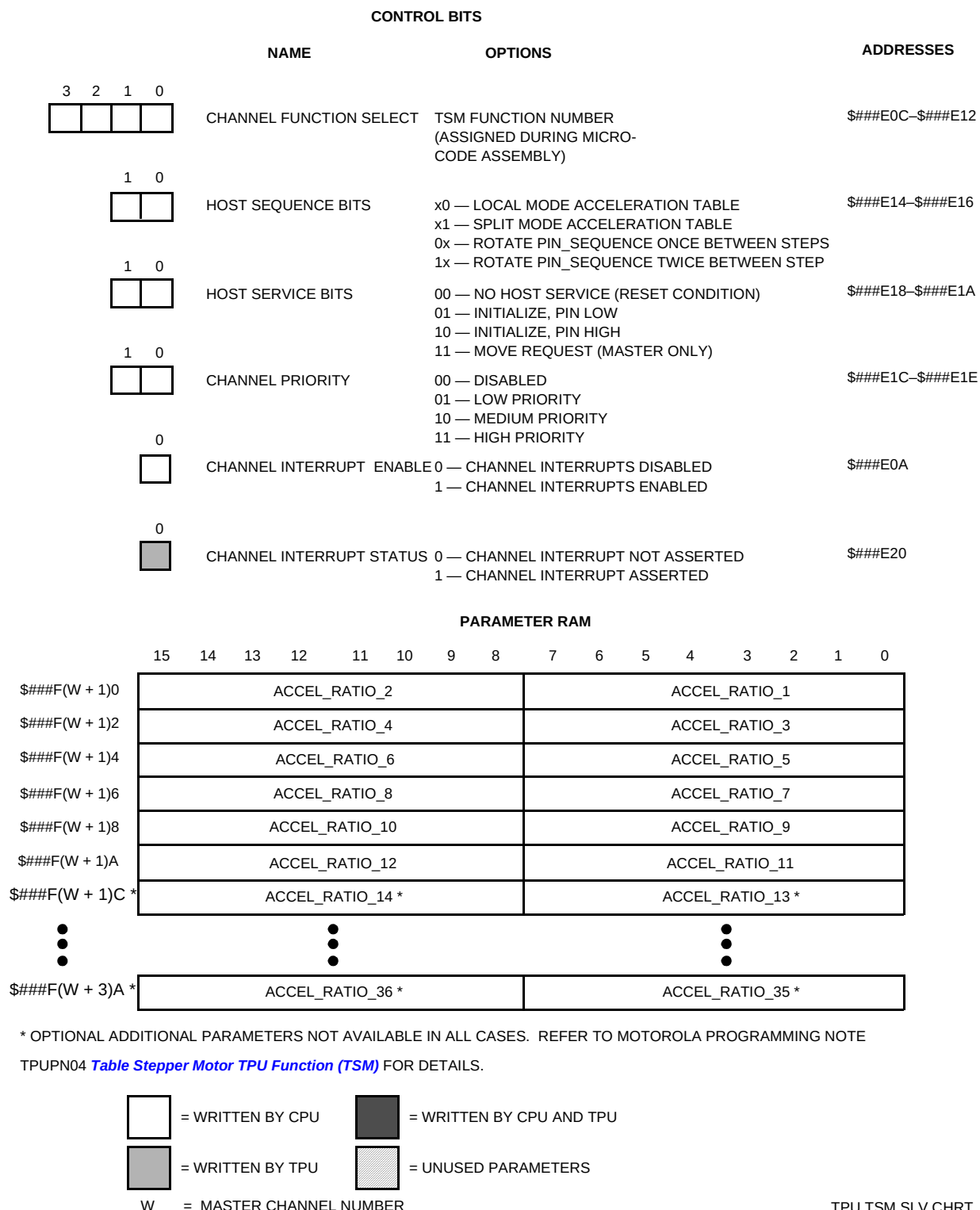
Figure D-5 TSM Parameters — Slave Mode
