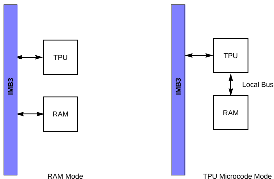
Figure 9-1 DPTRAM Configuration
