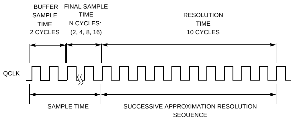
Figure 5-5 Conversion Timing
