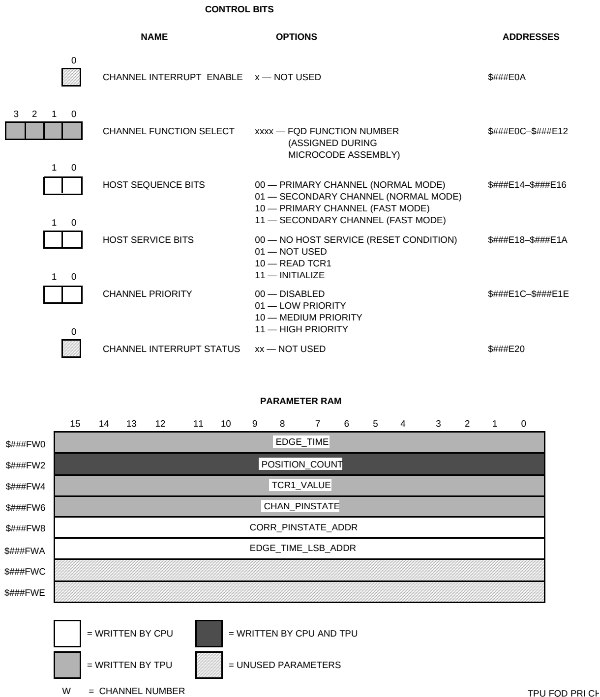
Figure D-19 FQD Parameters — Primary Channel
