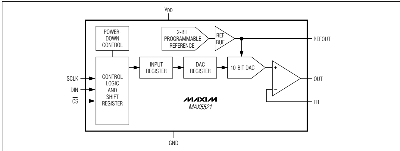
MAX5521 Functional Diagram
