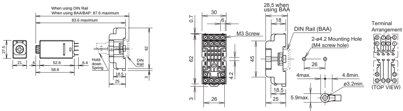
GT5Y Timer, Blade with SY4S-05
