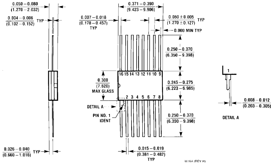
16-Lead Ceramic Flat Package (W) Order Number 54165FMQB NS Package Number W16A
