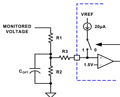
FIGURE 13. OV HYSTERESIS
