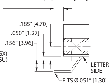
RIGHT ANGLE, DIP SOLDER (RA, SA)
