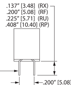
WIDE DIP SOLDER (RF, RX, RU, RP)
