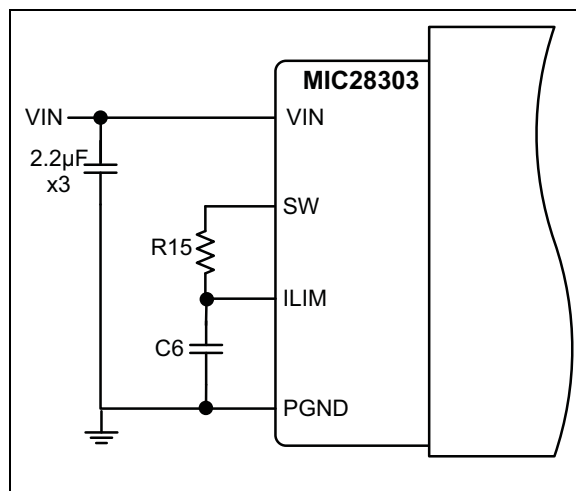
FIGURE 4-4: Current-Limiting Circuit
