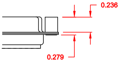
03X..... 0.236" (MATING SIDE) - CN8
