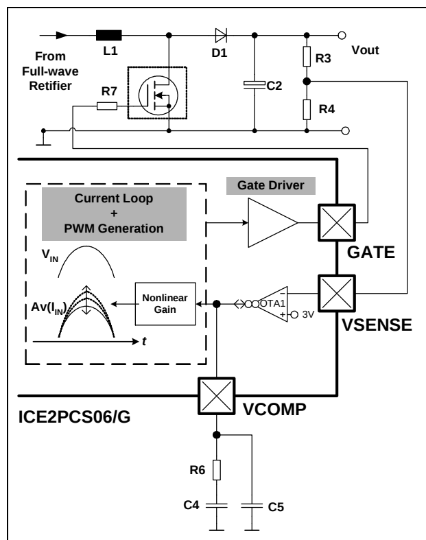
Figure 14 Voltage Loop
