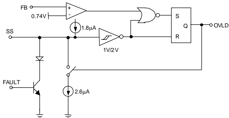
Figure 3. Details of the Soft-Start and Overload Hiccup Control Circuit
