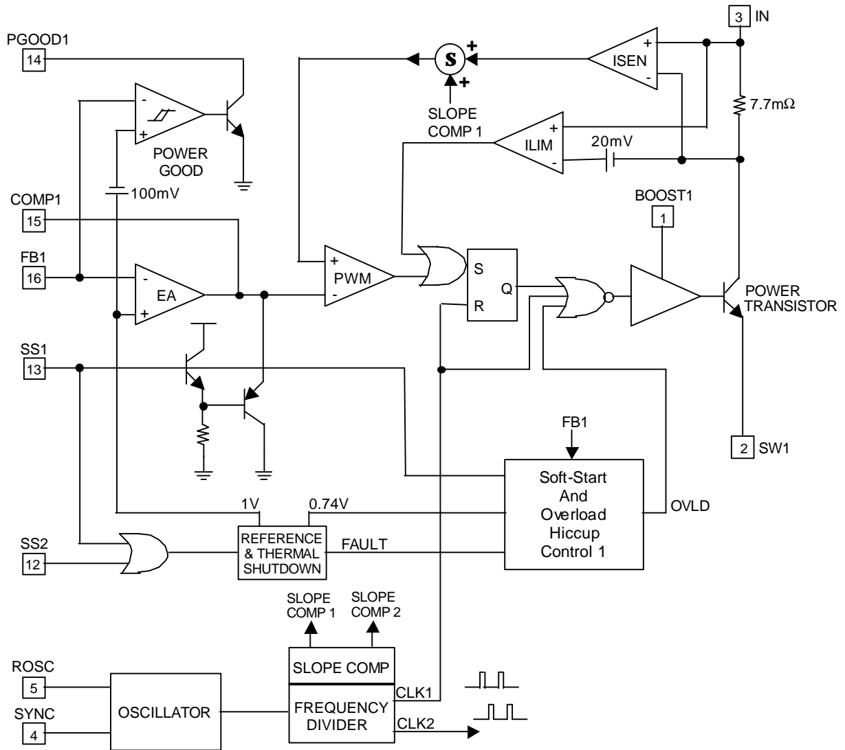
Figure 2. SC2440 Functional Diagram (One of Two Converters Shown)
