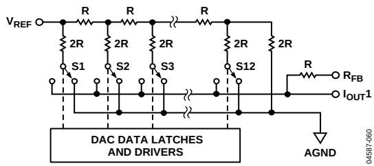
Figure 43. AD5452 Simplified Ladder
