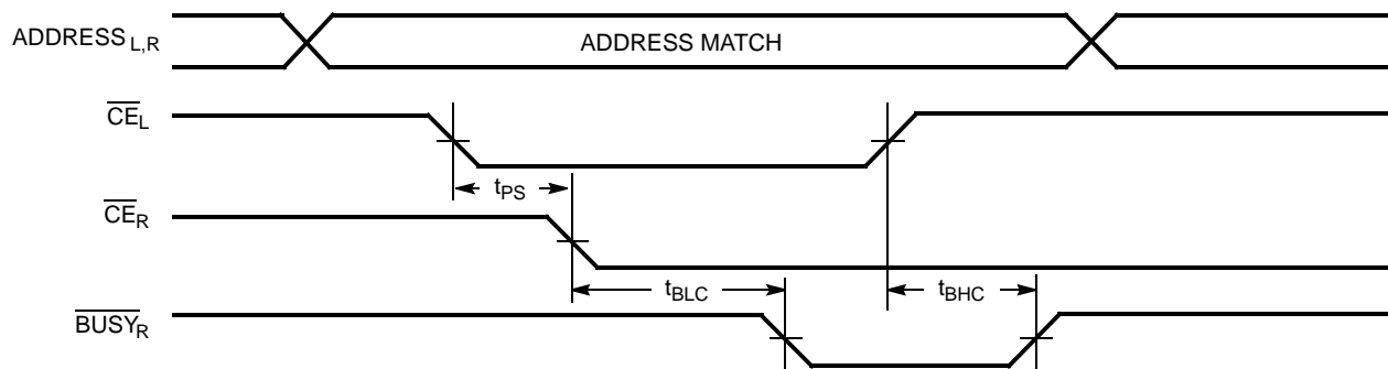
Figure 13. Busy Timing Diagram No. 1 ( \overline{\text{CE}} Arbitration) [42]
