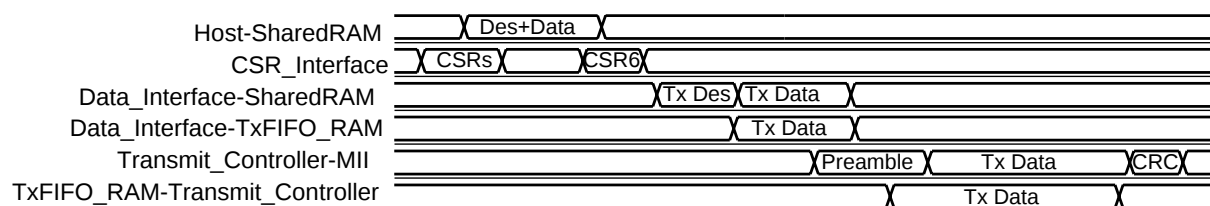
Figure 10 Transmit Data Flow
