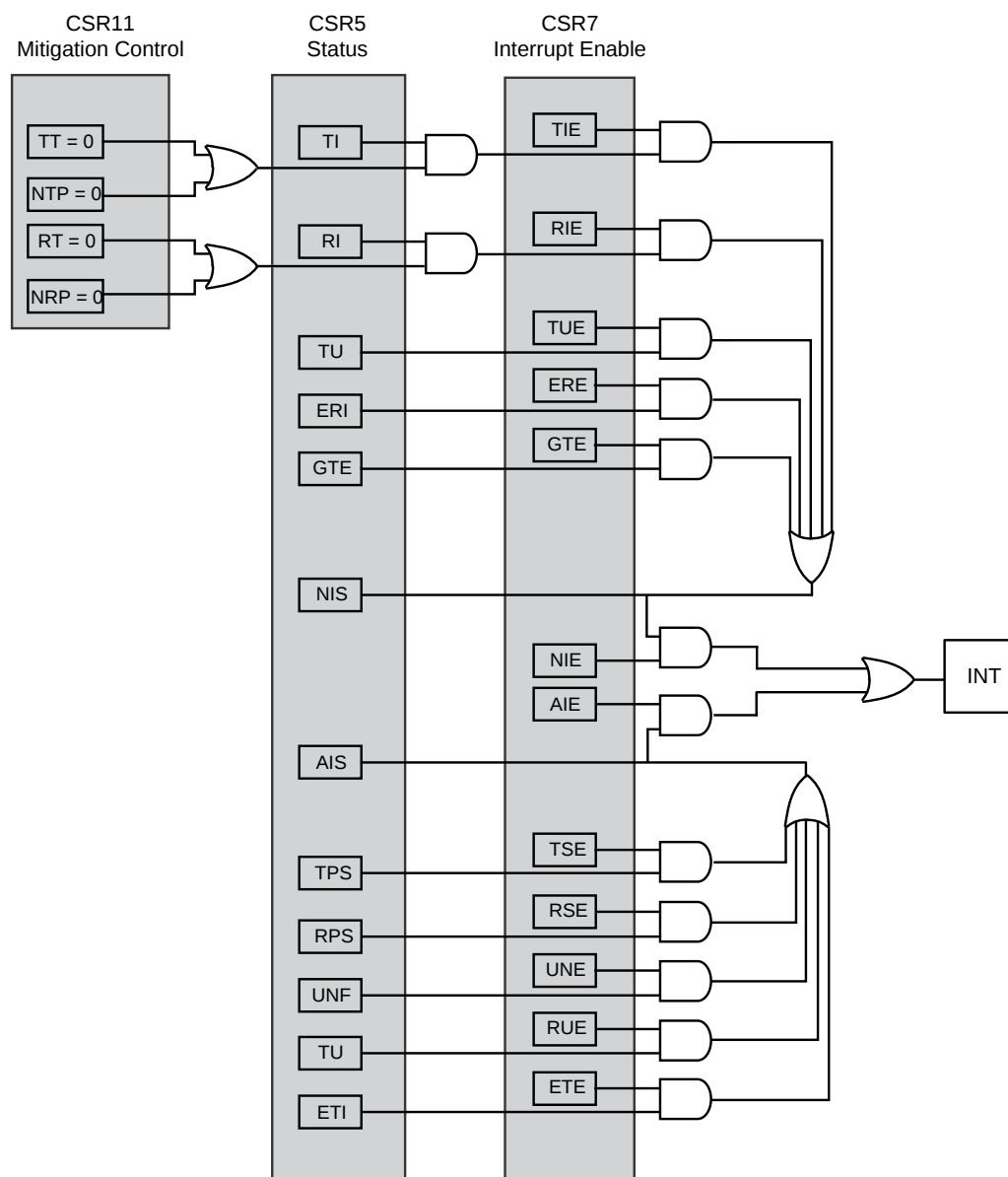
Figure 13 Interrupt Scheme
