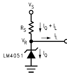
Figure 8-1. Shunt Regulator
