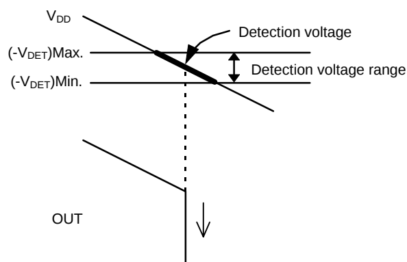
Figure 5 Detection Voltage
