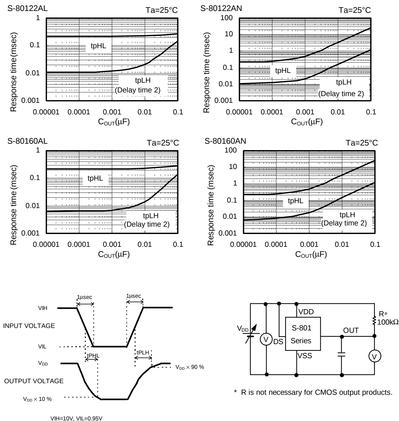
Figure 15 Measuring Conditions of Response Time
