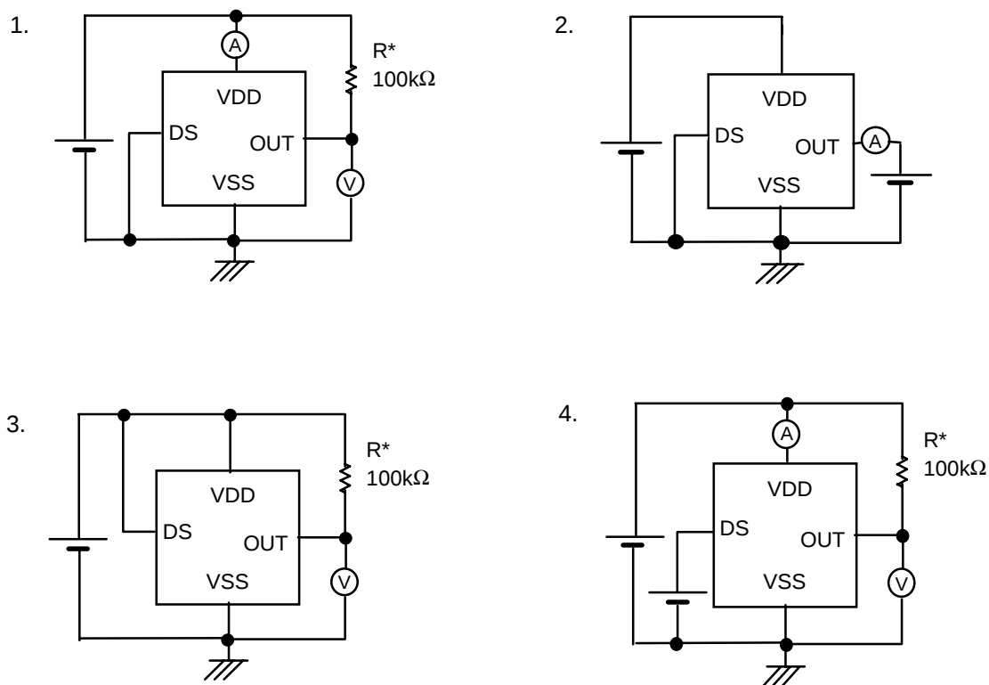
Figure 4 Test Circuits
