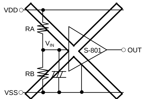
Figure 8 Misimplementation with Input Voltage Divider
