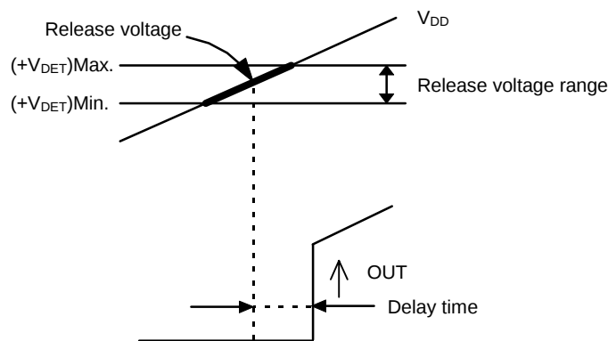
Figure 6 Release Voltage
