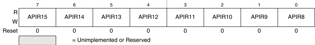
Figure 10-20. Autonomous Periodical Interrupt Rate High Register (CPMUAPIRH)
