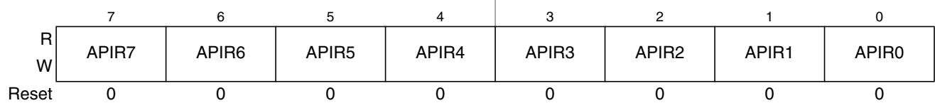
Figure 10-21. Autonomous Periodical Interrupt Rate Low Register (CPMUAPIRL)
