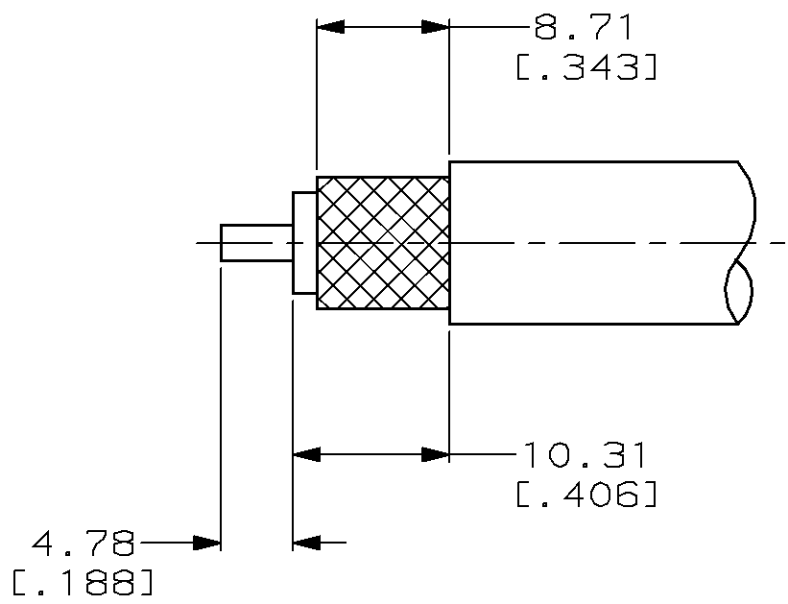
RECOMMENDED STRIP LENGTH (SCALE 2:1)
