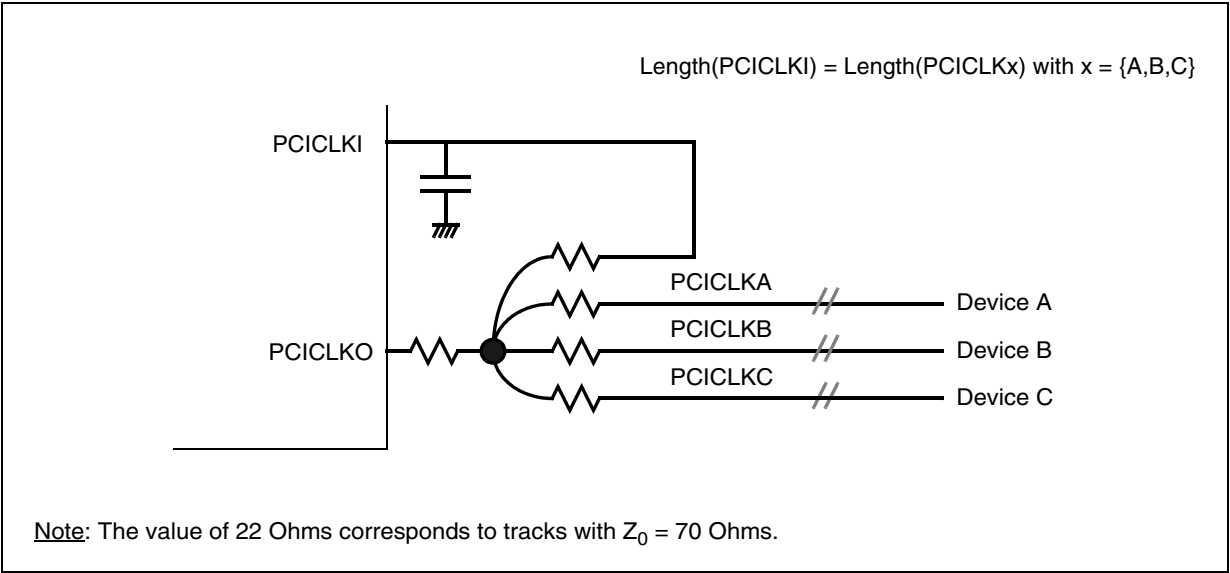
Figure 6-30. Clocks relationships
