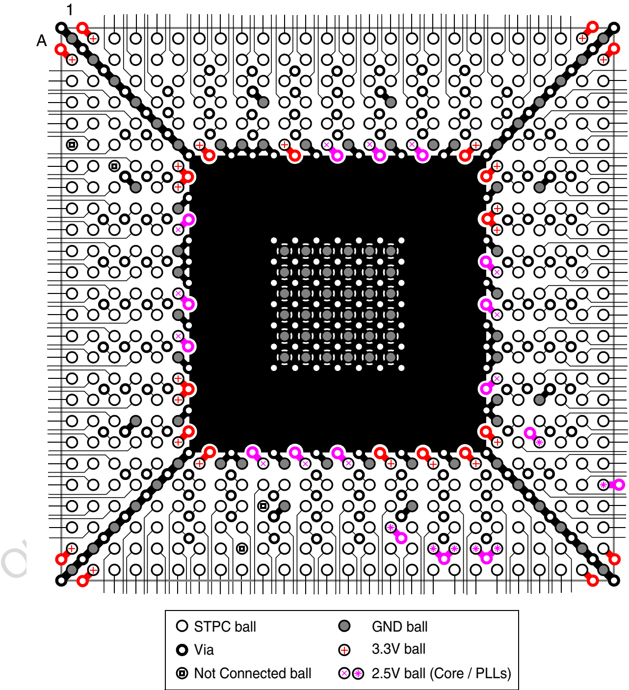
Figure 6-36. Layout for Good Thermal Dissipation - top layer
