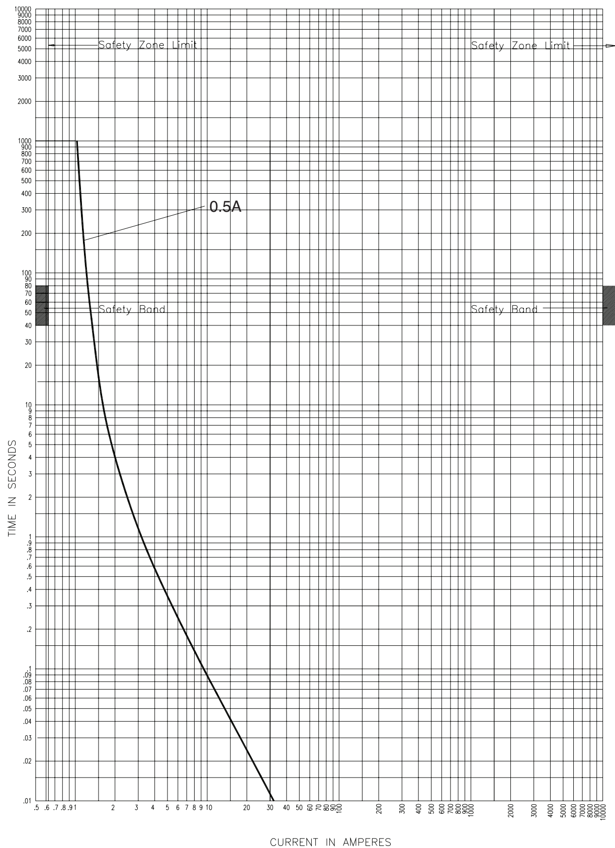
38kVTime-current curves — minimum melting for 38CLPT_
