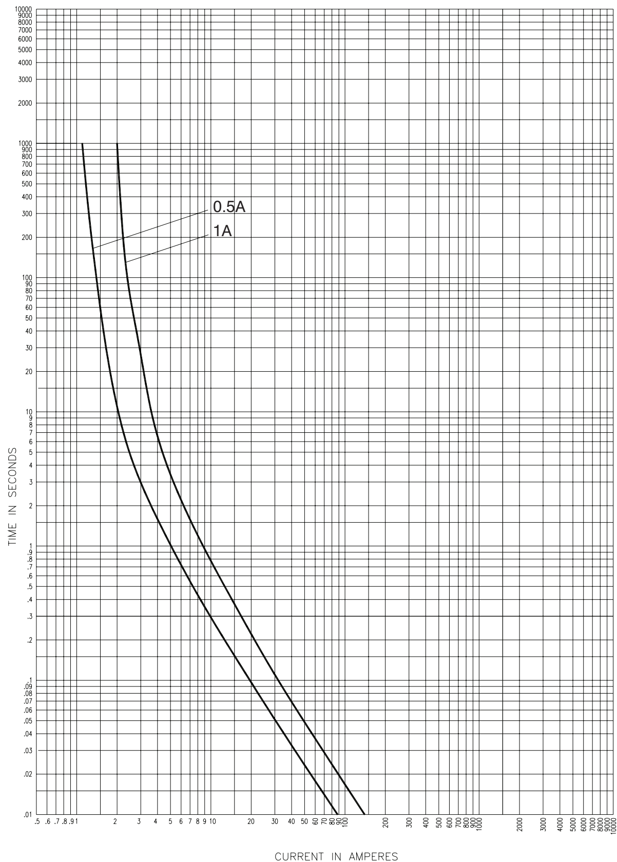
25.5kV Time-current curves — total clearing for 25CLPT_
