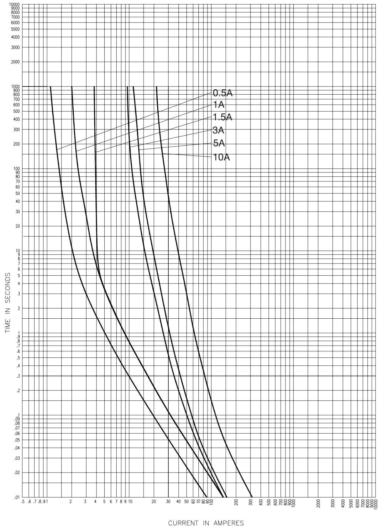
15.5kV Time-current curves — total clearing for 15CLPT_
