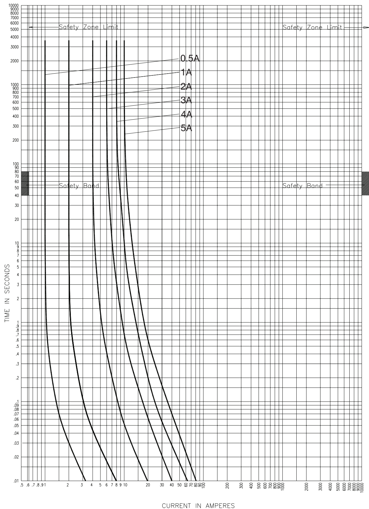
5.5kVTime-current curves — minimum melting for 5NCLPT_
