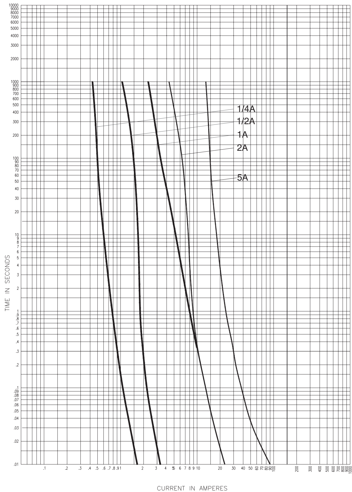
2.47kV Time-current curves — total clearing for 2NCLPT_E
