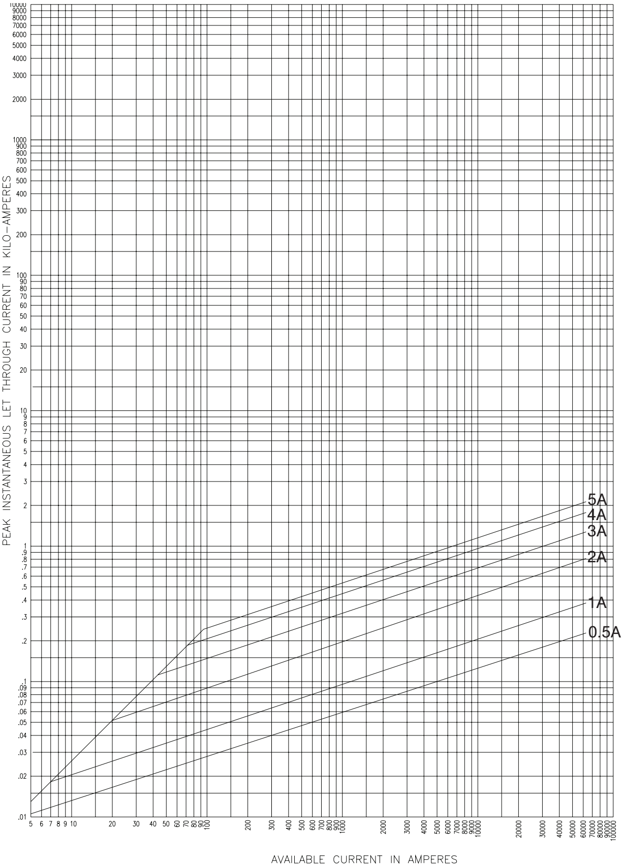
5.5kV Peak let-through curves for 5NCLPT_
