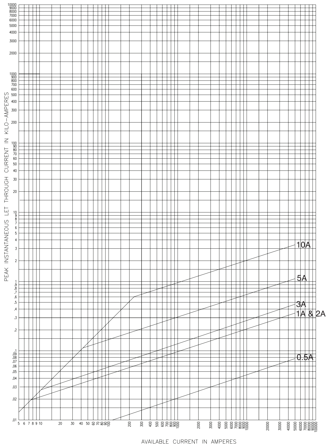
8.3kV Peak let-through curves for 8NCLPT_E-A/B
