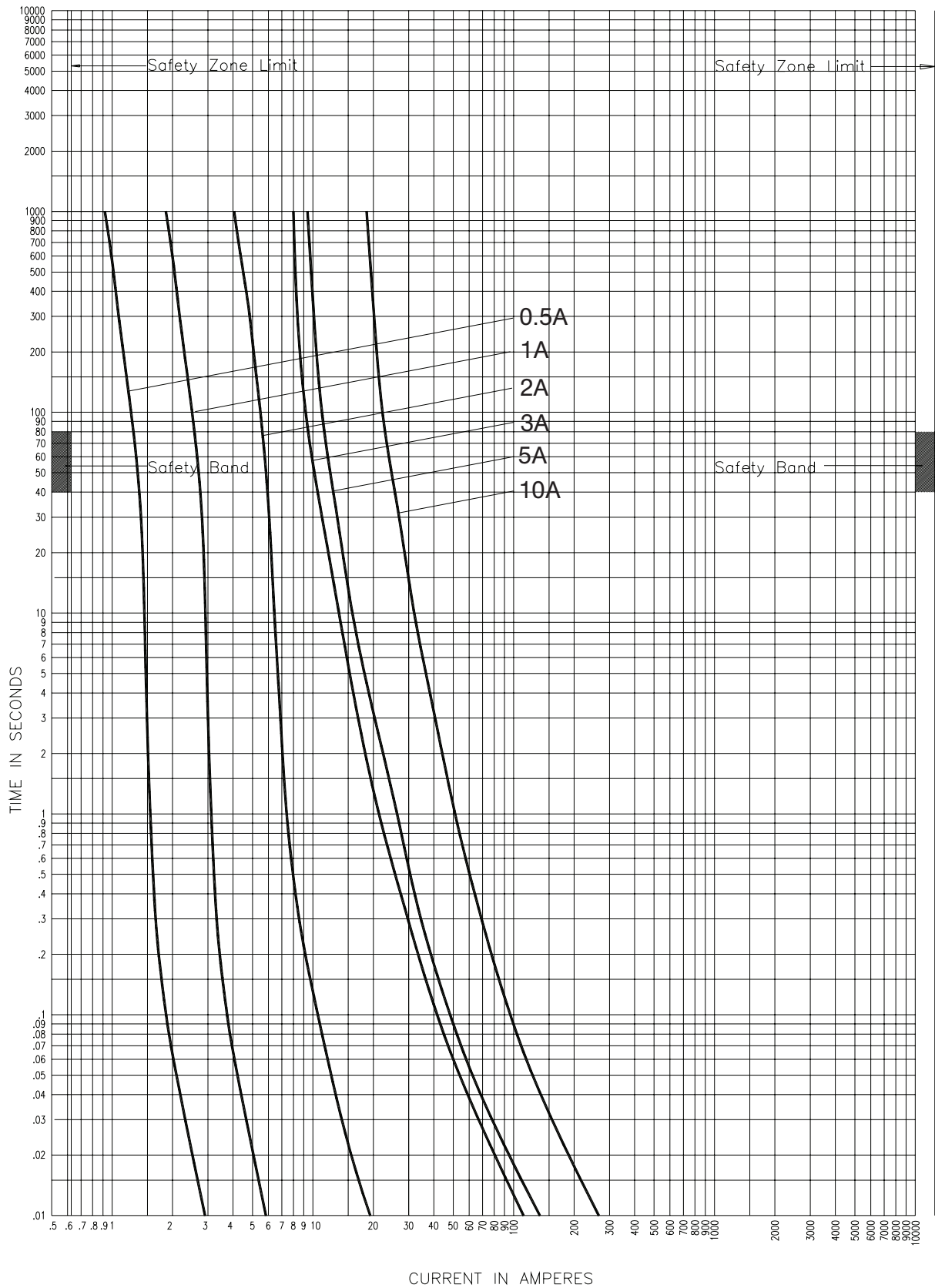
15.5kV Time-current curves — minimum melting for 15NCLPT_
