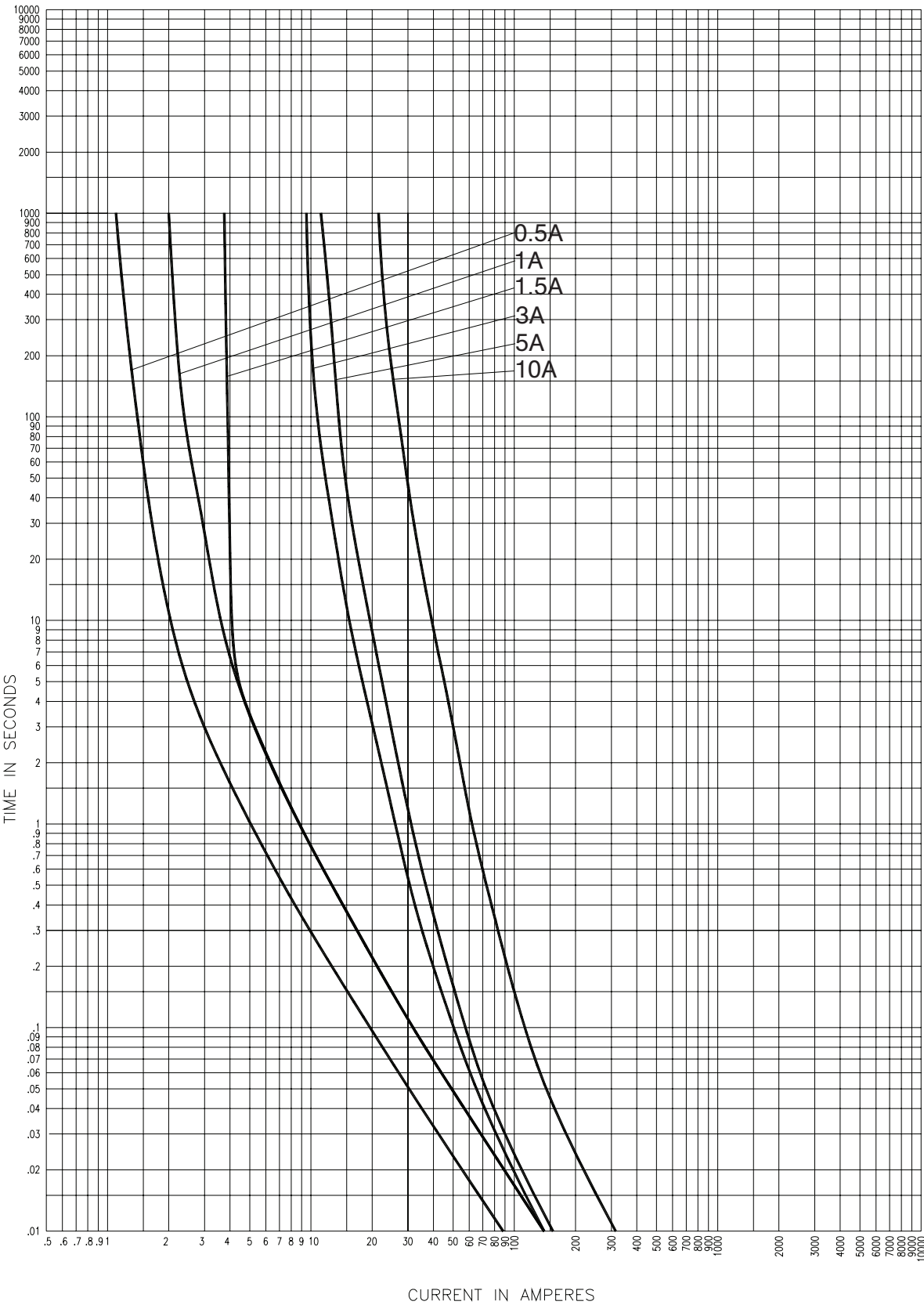
5.5kV Time-current curves — total clearing for 5CLPT_
