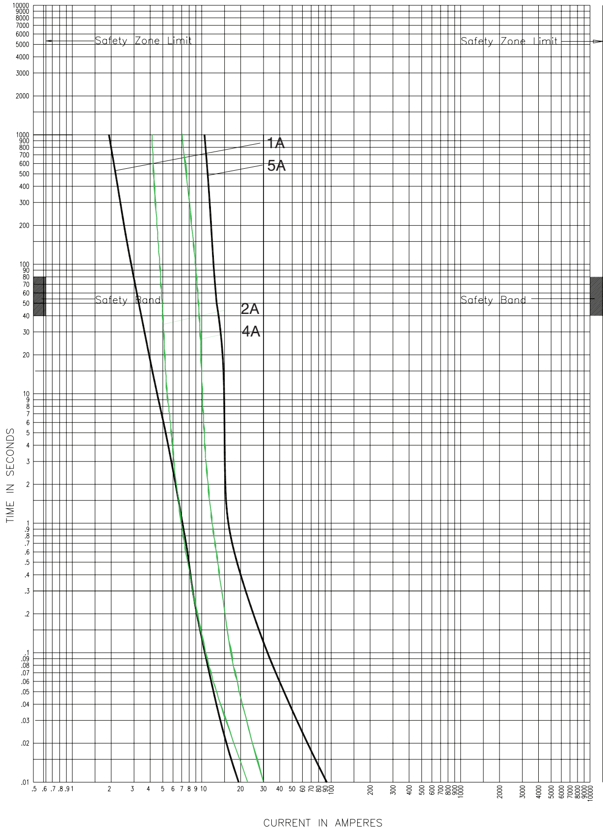
8.3kVTime-current curves — minimum melting for 8NCLPT_
