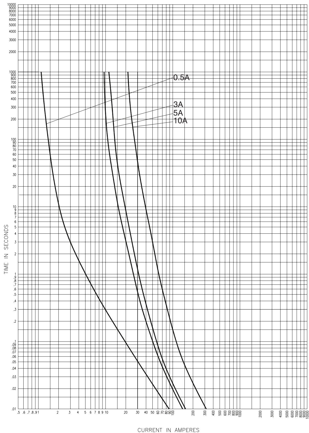
8.3kVTime-current curves — total clearing for 8CLPT_
