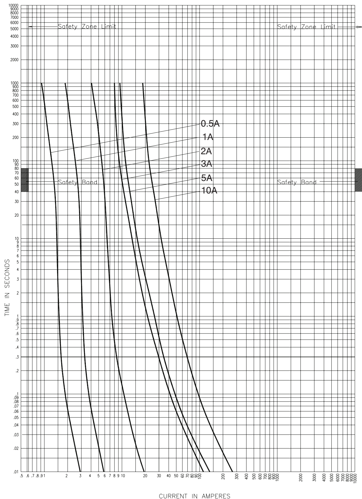
8.3kV Time-current curves — minimum melting for 8NCLPT_E-A/B
