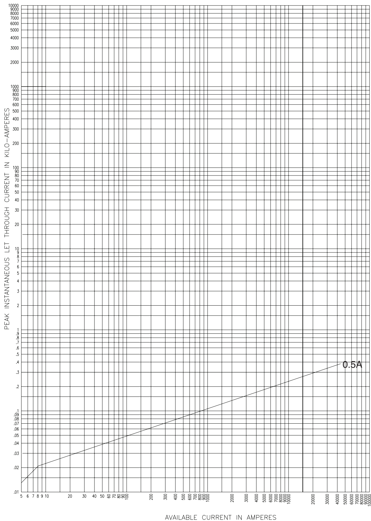
38kV Peak let-through curves for 38CLPT_
