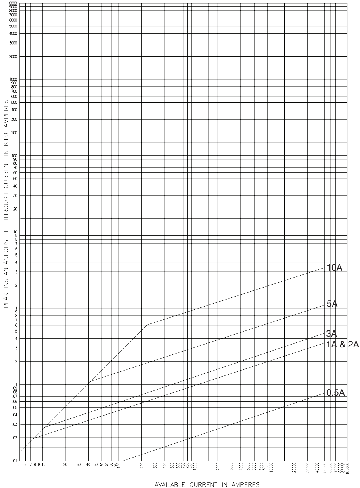
15.5kV Peak let-through curves for 15NCLPT_
