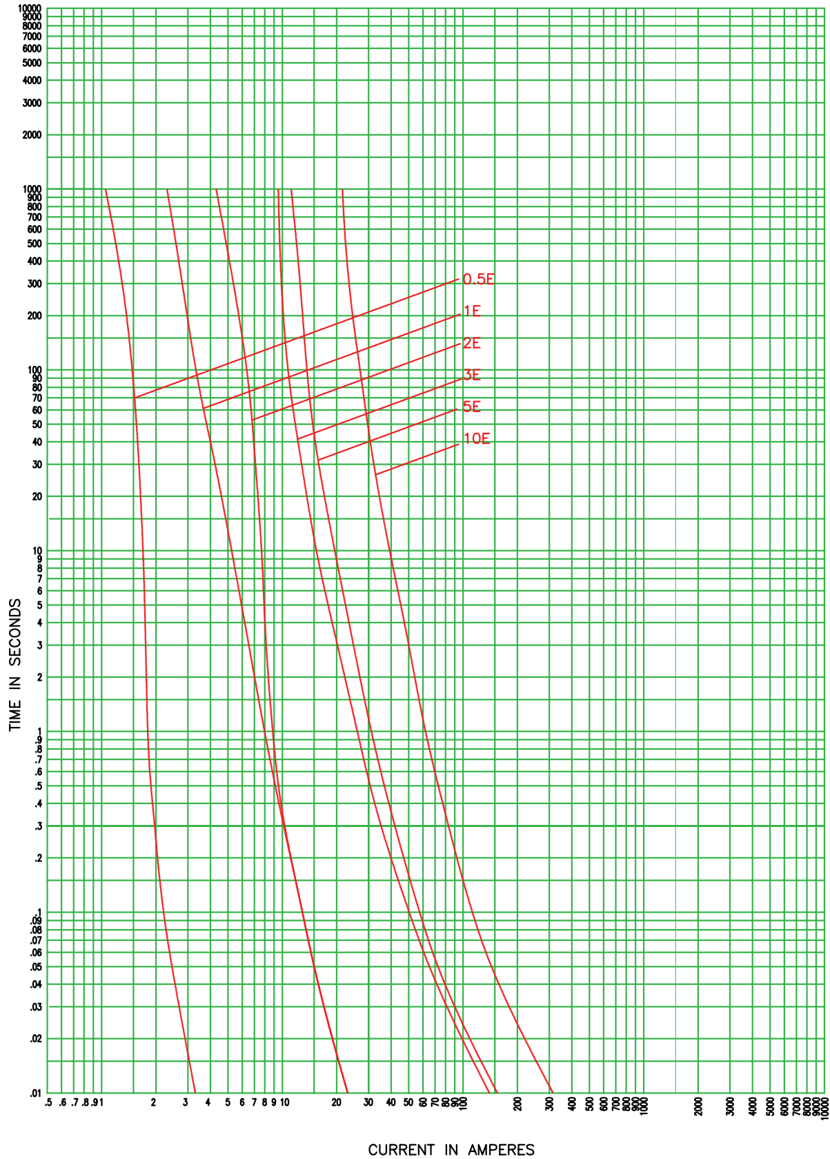
5.5kVTime-current curves — total clearing for 5NCLPT_-A
