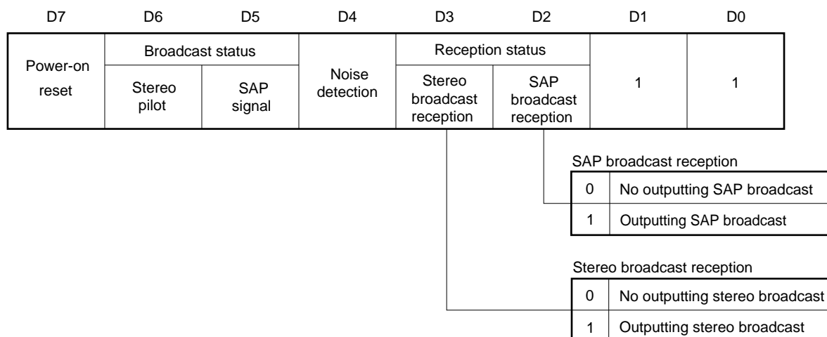
Figure 4-7. Stereo, SAP Broadcast Reception (Reception Status) Detection
