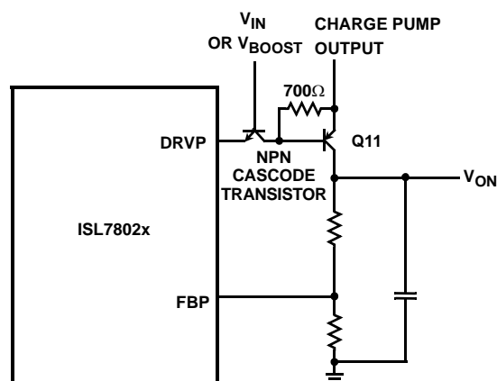
FIGURE 20. CASCODE NPN TRANSISTOR CONFIGURATION FOR HIGH CHARGE PUMP OUTPUT VOLTAGE (&gt;36V)
