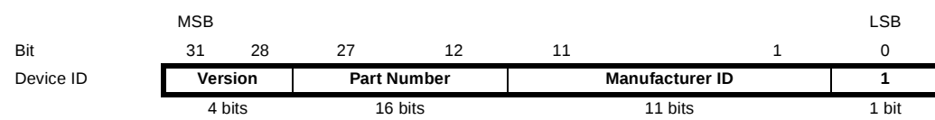
Figure 87. The format of the Device Identification Register
