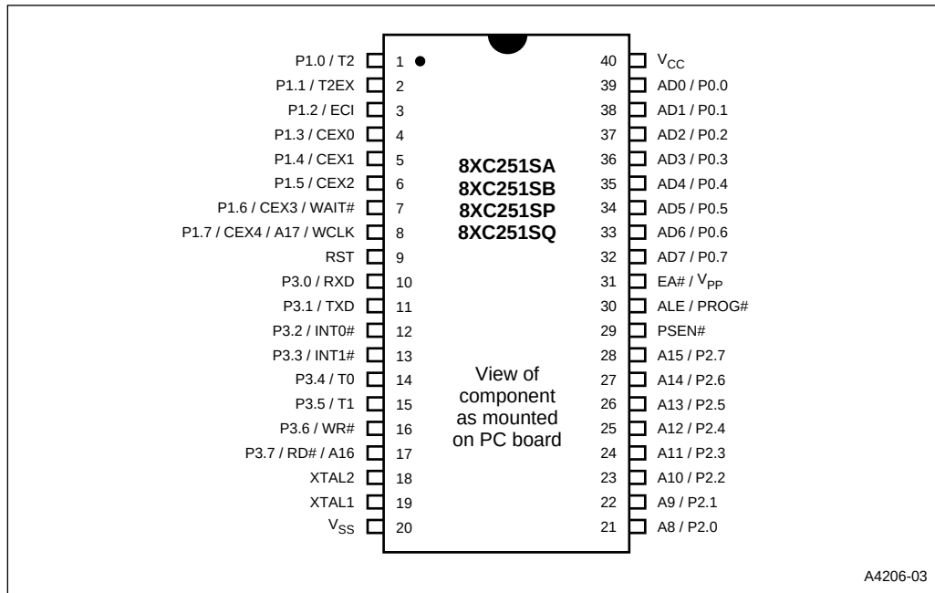
Figure 4. 8XC251SA/SB/SP/SQ 40-lead PDIP and Ceramic DIP Packages
