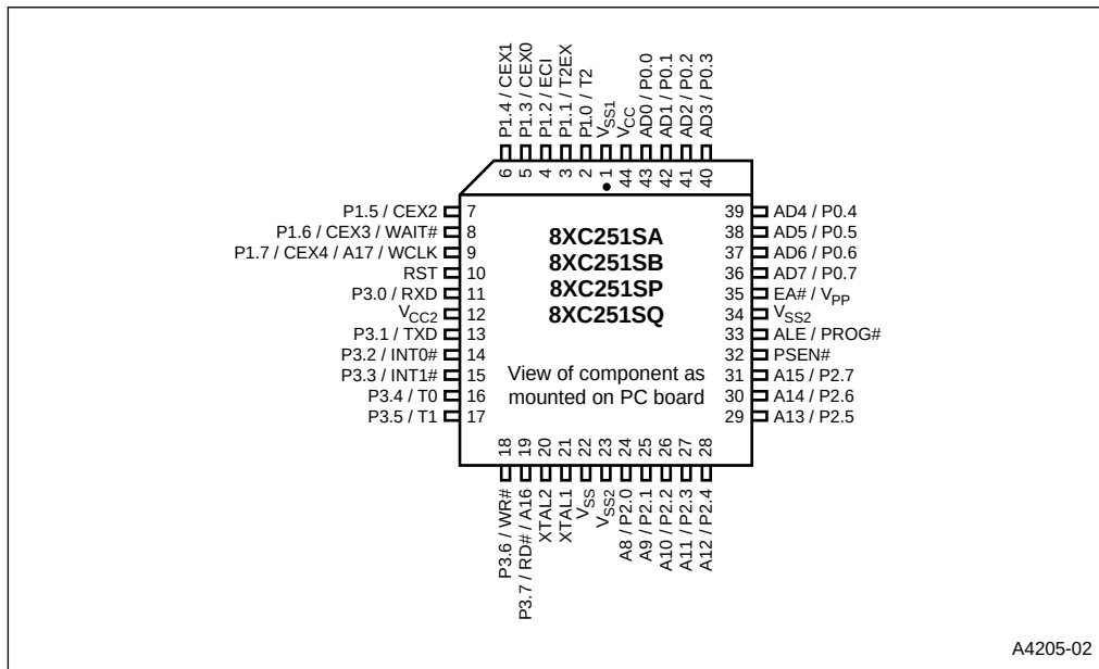
Figure 3. 8XC251SA/SB/SP/SQ 44-lead PLCC Package
