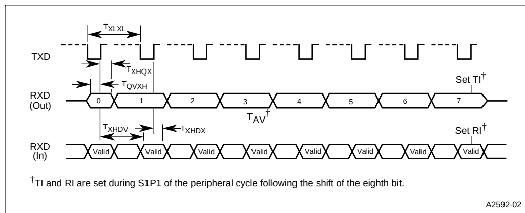
Figure 12. Serial Port Waveform — Shift Register Mode
