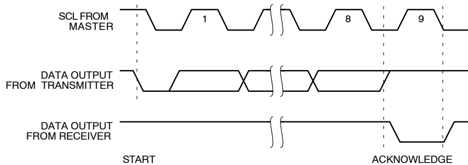
Figure 6. Acknowledge Timing
