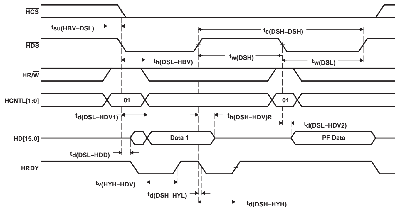
Figure 36. Multiplexed Read Timings Without \overline{H\bar{A}S}
