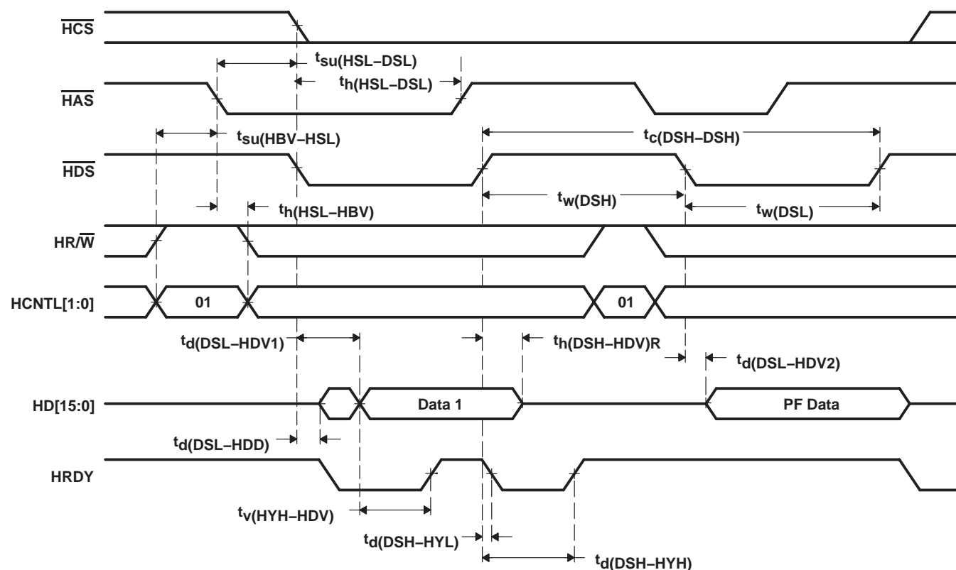
Figure 35. Multiplexed Read Timings Using \overline{H\bar{A}S}
