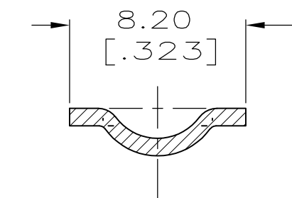
SECTION C-C
