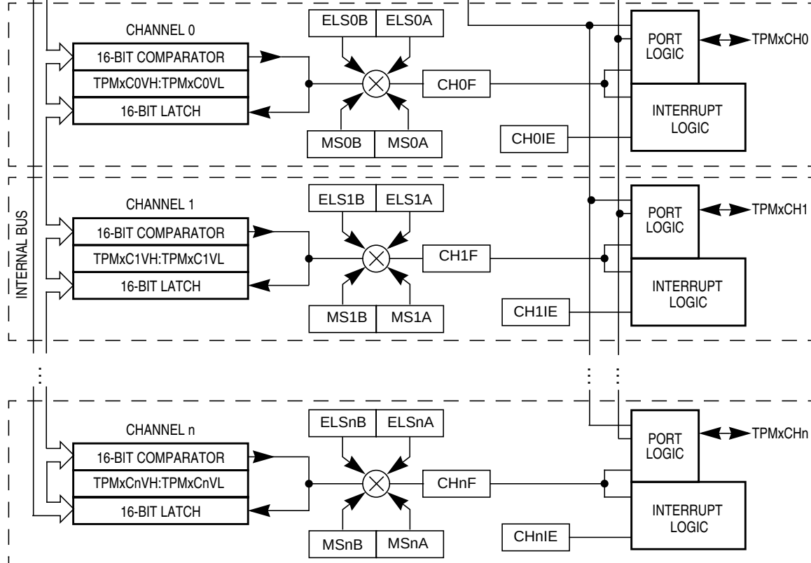
Figure B-1. TPM Block Diagram
