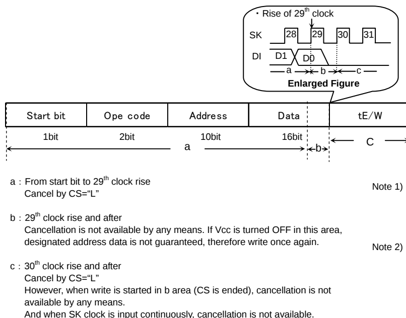
Figure 35. Write, WrAl Cancel Available Timing
