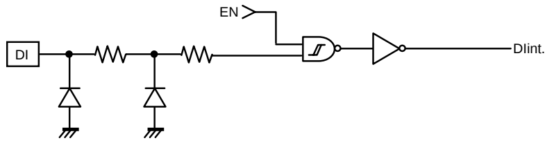
Figure 39. Input Circuit (DI)
