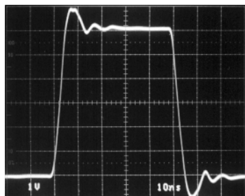
Large-Signal Transient, A_V = -1, V_S = \pm 5V
