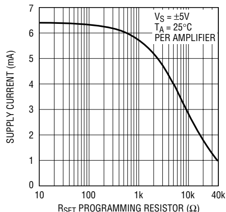
Supply Current vs Programming Resistor
