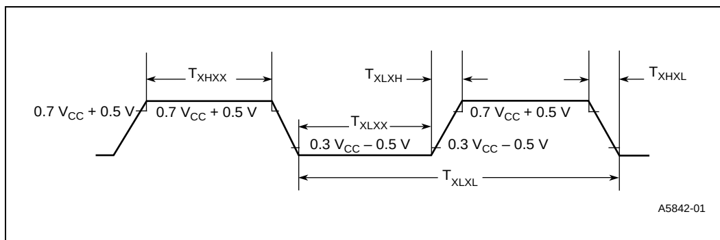
Figure 11. External Clock Drive Waveforms
