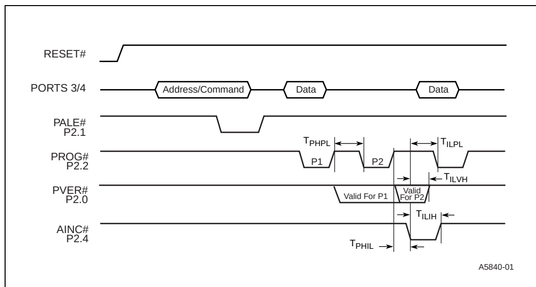
Figure 16. Slave Programming Mode Timing in Data Program Mode with Repeated PROG Pulse and Auto Increment
