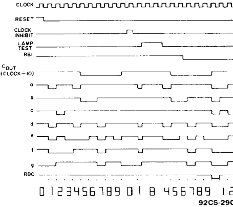
Fig. 4 – CD4033B timing diagram.
