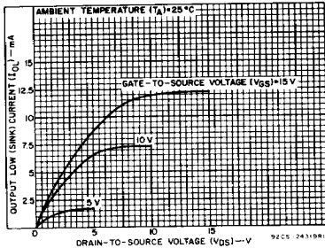
Fig. 7 – Minimum n-channel output low (sink) current characteristics.
