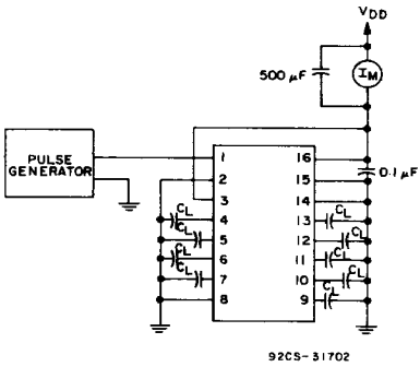
Fig. 14 – Dynamic power dissipation test circuit for CD4033B.
