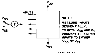
Fig. 17 – Input current.
