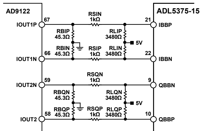
Figure 67. Passive Level-Shifting Network For Biasing ADL5375-15 from TxDAC
