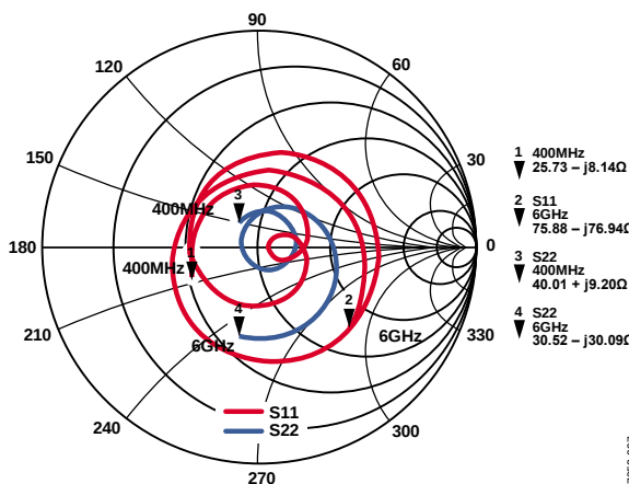
Figure 7. Smith Chart of LOIP (LOIN AC-Coupled to Ground) S11 and RFOUT S22 from 450 MHz to 6000 MHz
