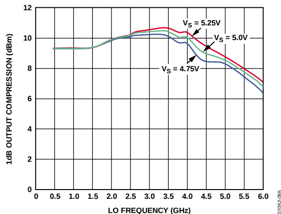
Figure 6. SSB Output 1dB Compression Point ( \text{OP1dB} ) vs. LO Frequency ( f_{\text{LO}} ) and Supply
