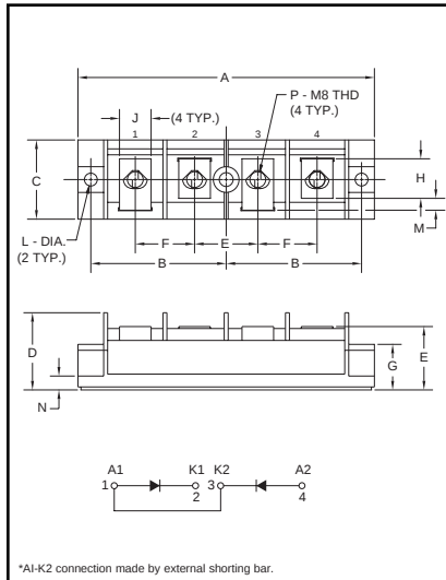
Outline Drawing
