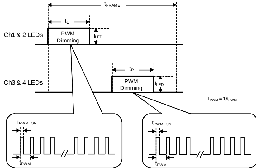
FIGURE 15. 3D APPLICATION TIMING DIAGRAM
