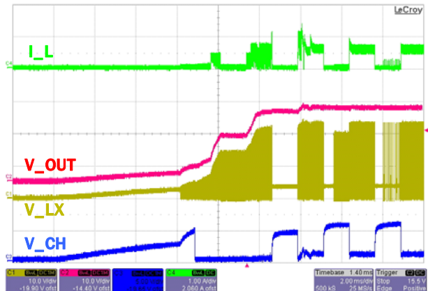
FIGURE 8. START-UP (50% DIRECT PWM DIMMING, V_{IN} = 3.7V , I_{CH} = 20mA , f_{DIM} = 200Hz , LEDs = 4P7S)
